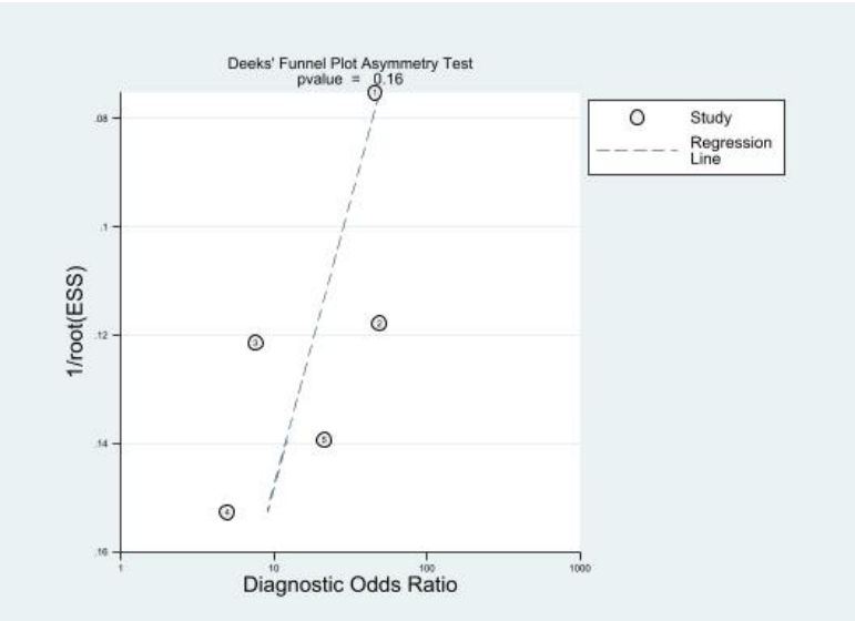
Supplementary Fig. 9. Linear regression test of funnel plot asymmetry.
