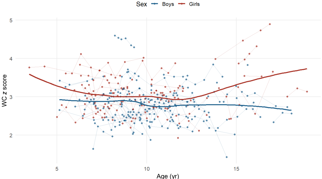
Supplementary Fig. 2. Waist circumference (WC) z score trajectories by age and sex. Each dot represents an individual visit, and connecting lines indicate repeated measurements from the same participant. Smoothed trajectories (locally estimated scatterplot smoothing) are shown separately by sex.
